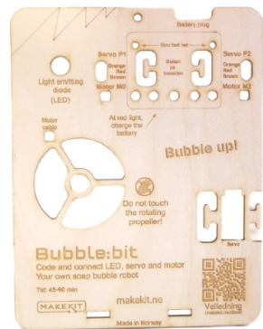
Monteringsplate
